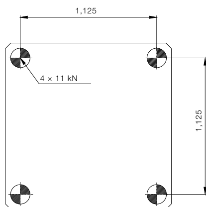
Foundation loading
