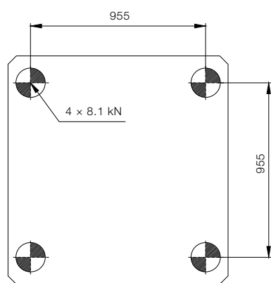
Foundation loading
