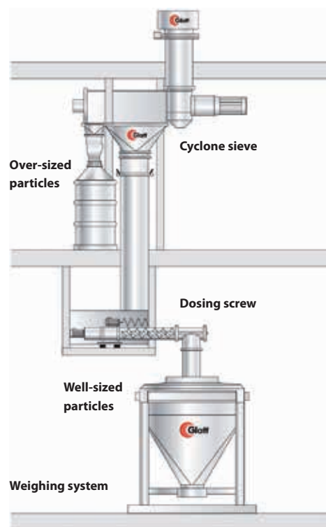
Dosing system with integrated cyclone sieve and dosing screw
