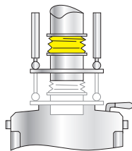
Static seal with pneumatic lifting device
