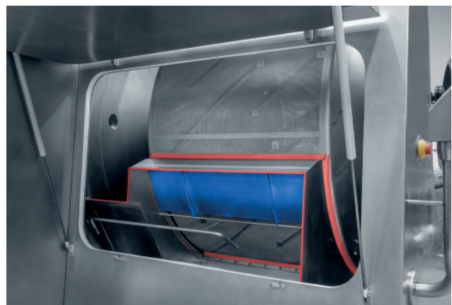
Exhaust air chamber with guide plate
